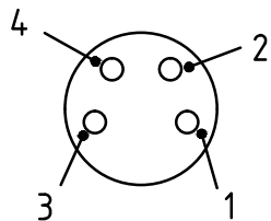
FEMALE END VIEW
